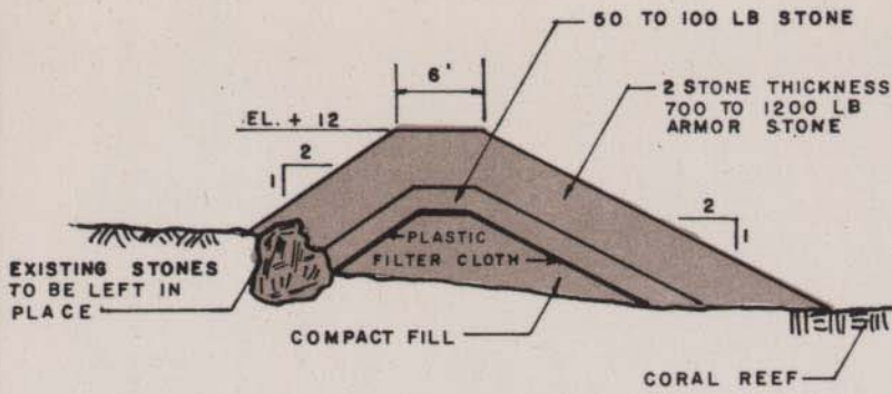
TYPICAL REVETMENT SECTION "A-A"
