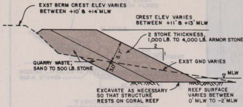
TYPICAL SECTION (REACHS A TO F)
