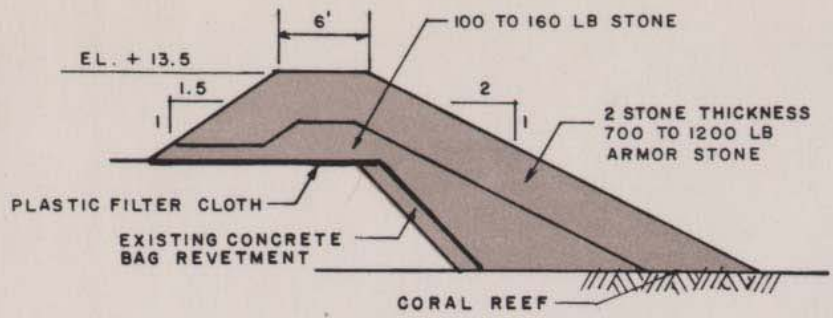
REVETMENT SECTION "A-A"
