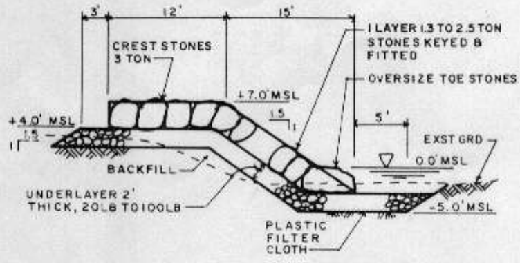
TYPICAL REVETMENT SECTION NOT TO SCALE
