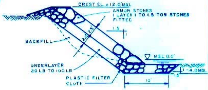
TYPICAL REVETMENT SECTION NOT TO SCALE
