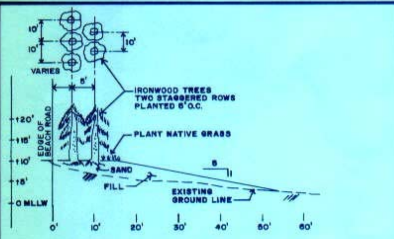
TYPICAL SHORE PROTECTION SECTION
