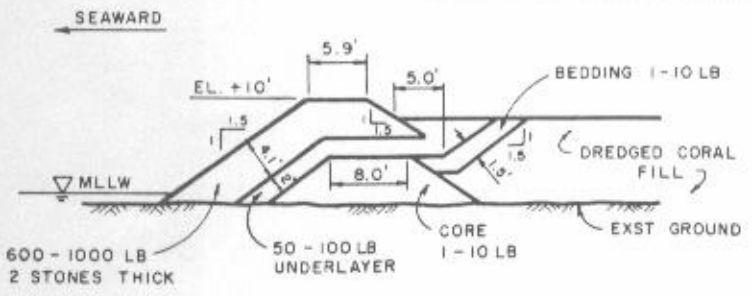
TYPICAL NORTH REVETTED MOLE SECTION NOT TO SCALE
