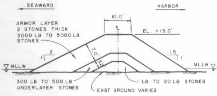
TYPICAL MAIN BREAKWATER SECTION NOT TO SCALE
