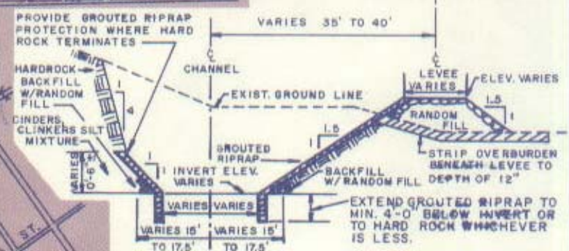
TYPICAL SECTION LEVEE & CHANNEL WAILOA F.C. CHANNEL NOT TO SCALE
