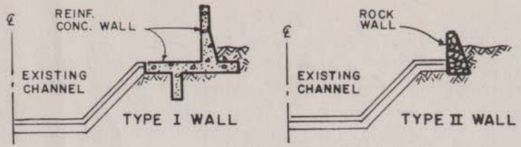
MODIFIED UPPER EXISTING CHANNEL
