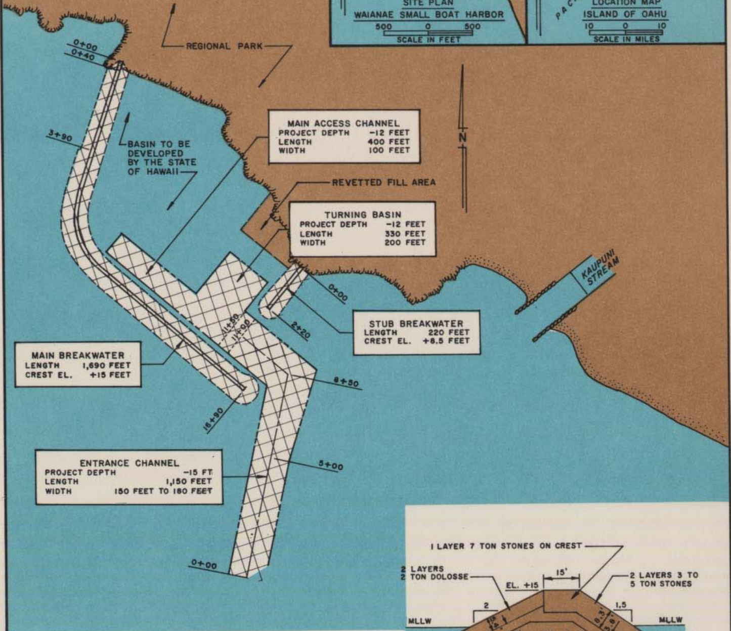
MAIN BREAKWATER 3+90 TO 16+90
