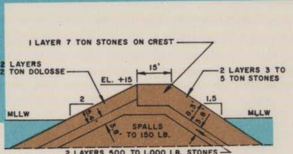
MAIN BREAKWATER 3+90 TO 16+90
