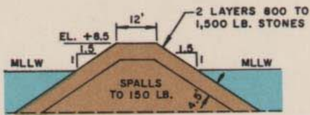
STUB BREAKWATER
