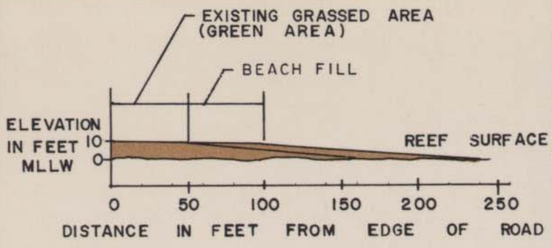
TYPICAL BEACH SECTION
